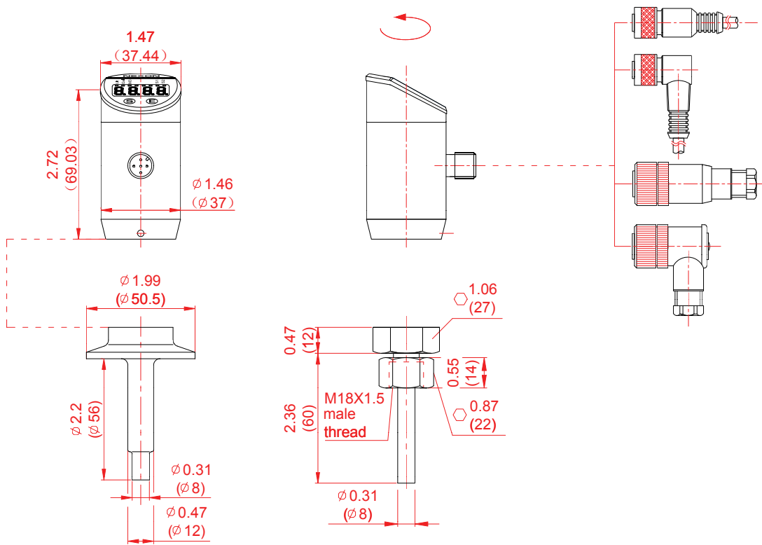
Probe with S50 thread (for the sanitary)
